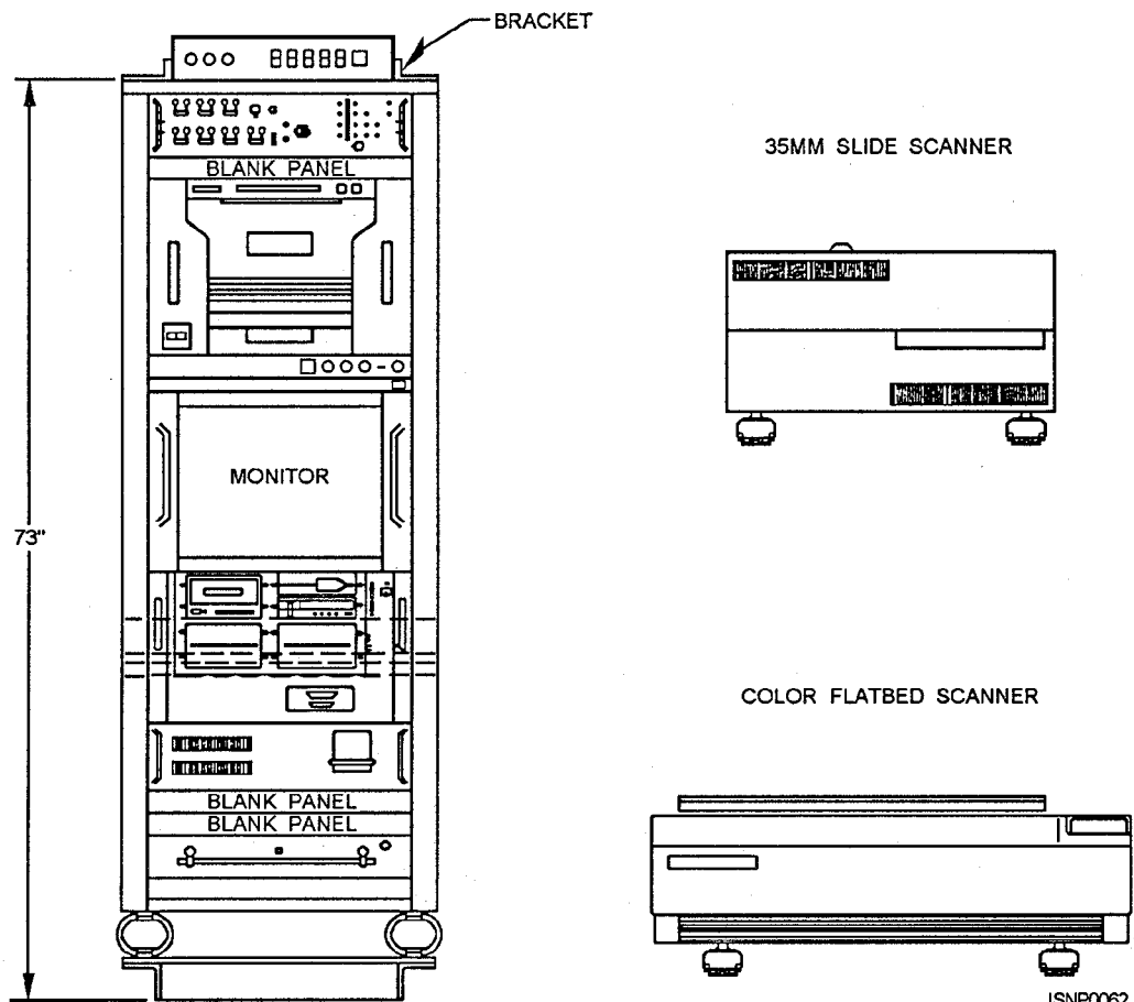
Figure 6-12.—PIES configuration.
